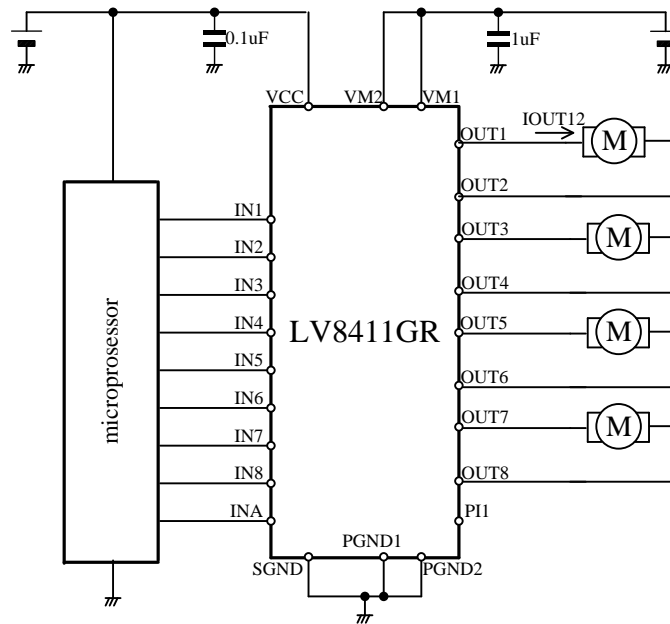
Figure 15. DC motor drive circuit
