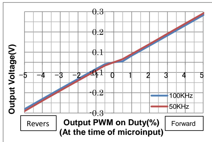
Figure 18. Input and Output Characteristics of H-Bridge
