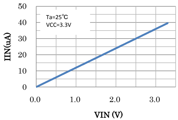
Figure 5. Input current vs. Input voltage
