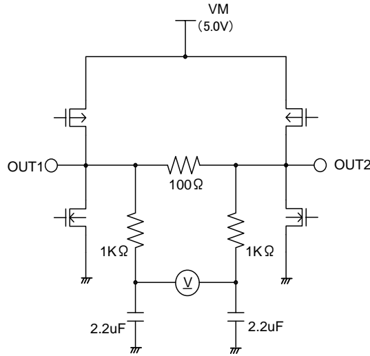
Figure 17. Measurement connection diagram
